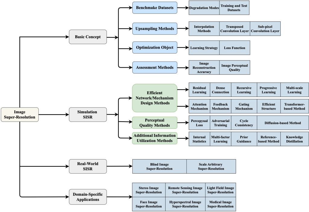
Fig. 2. The content and taxonomy of this survey. In this survey, we divide image SR methods into three categories: Simulation SISR, Real-World SISR, and Domain-Specific Applications.
