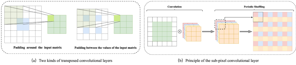
Fig. 4. Upsampling methods: (a) transposed convolutional layers (b) sub-pixel convolutional layer.
