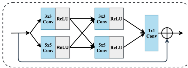
Fig. 8. The structure of multi-scale residual block (MSRB [98]).
