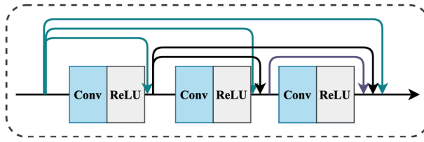
Fig. 6. The structure of the dense connection module.
