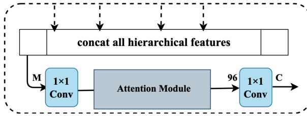
Fig. 10. The structure of the HFDB.
