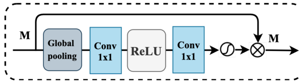
Fig. 9. The principle of CAM.
